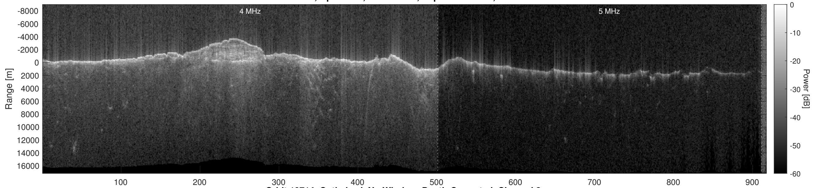
Orbit 10714, Optimized, No Window, Depth-Corrected, Channel 2
