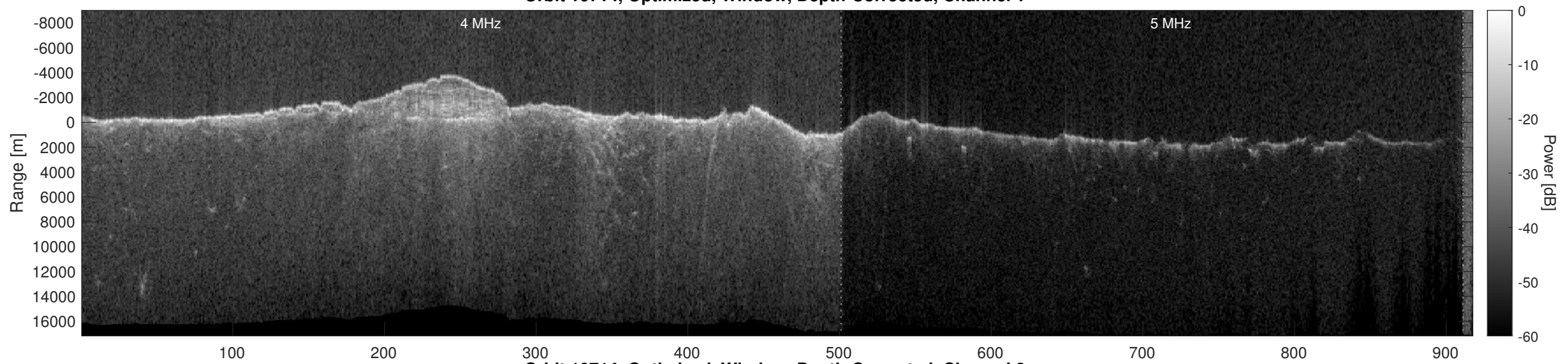
Orbit 10714, Optimized, Window, Depth-Corrected, Channel 2
