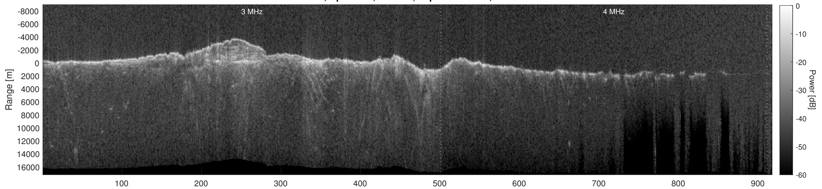
Orbit 10714, Depth-Corrected Cluttergram
