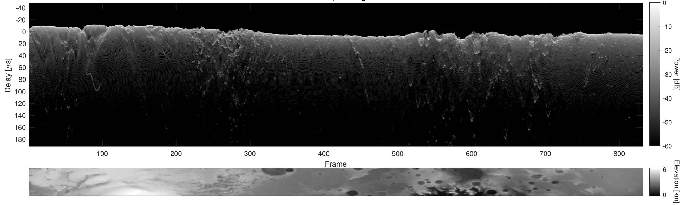
Orbit 10715, Cluttergram
