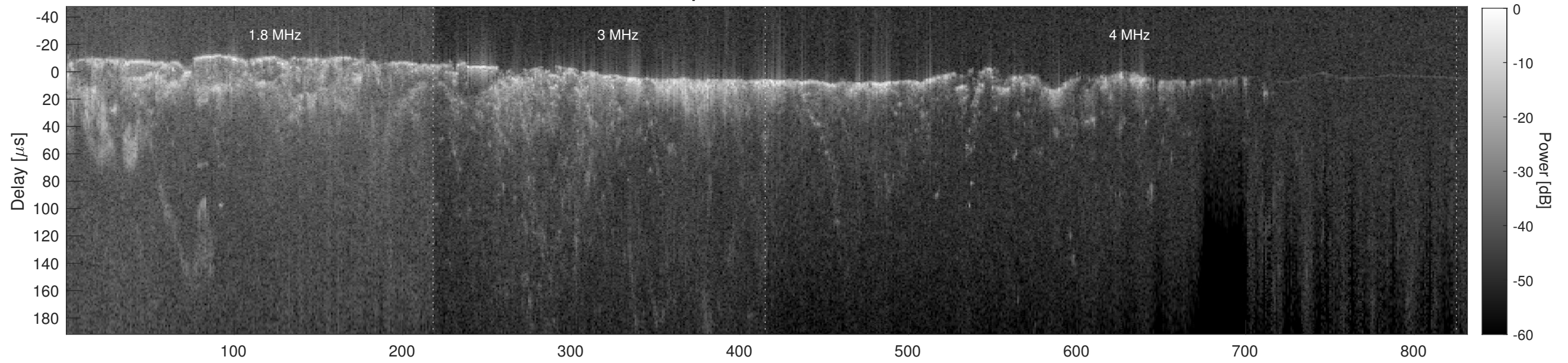
Orbit 10715, Cluttergram
