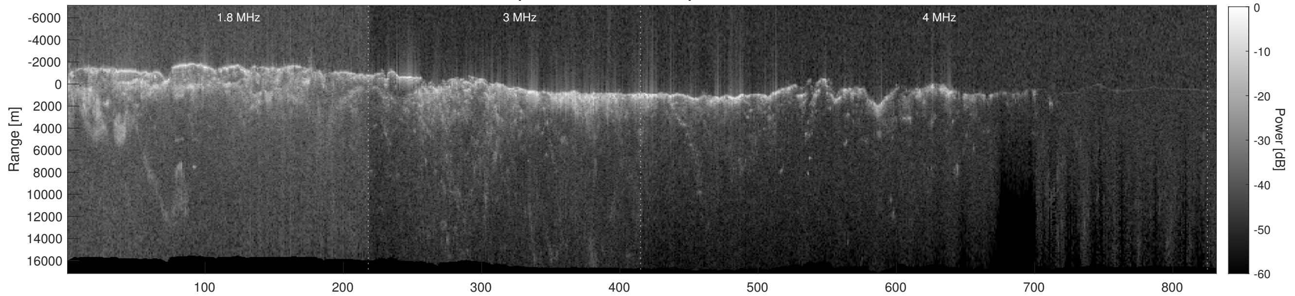
Orbit 10715, Depth-Corrected Cluttergram
