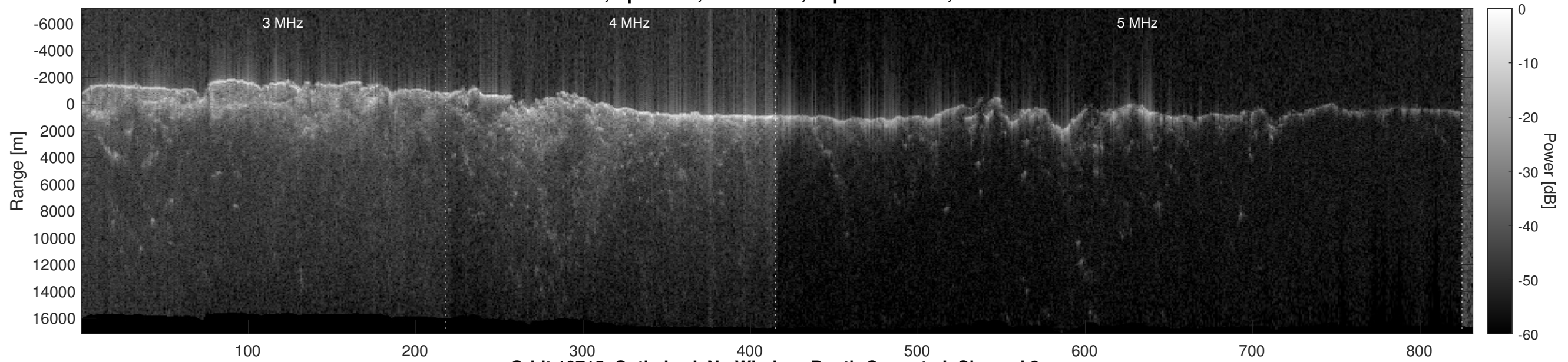
Orbit 10715, Optimized, No Window, Depth-Corrected, Channel 2
