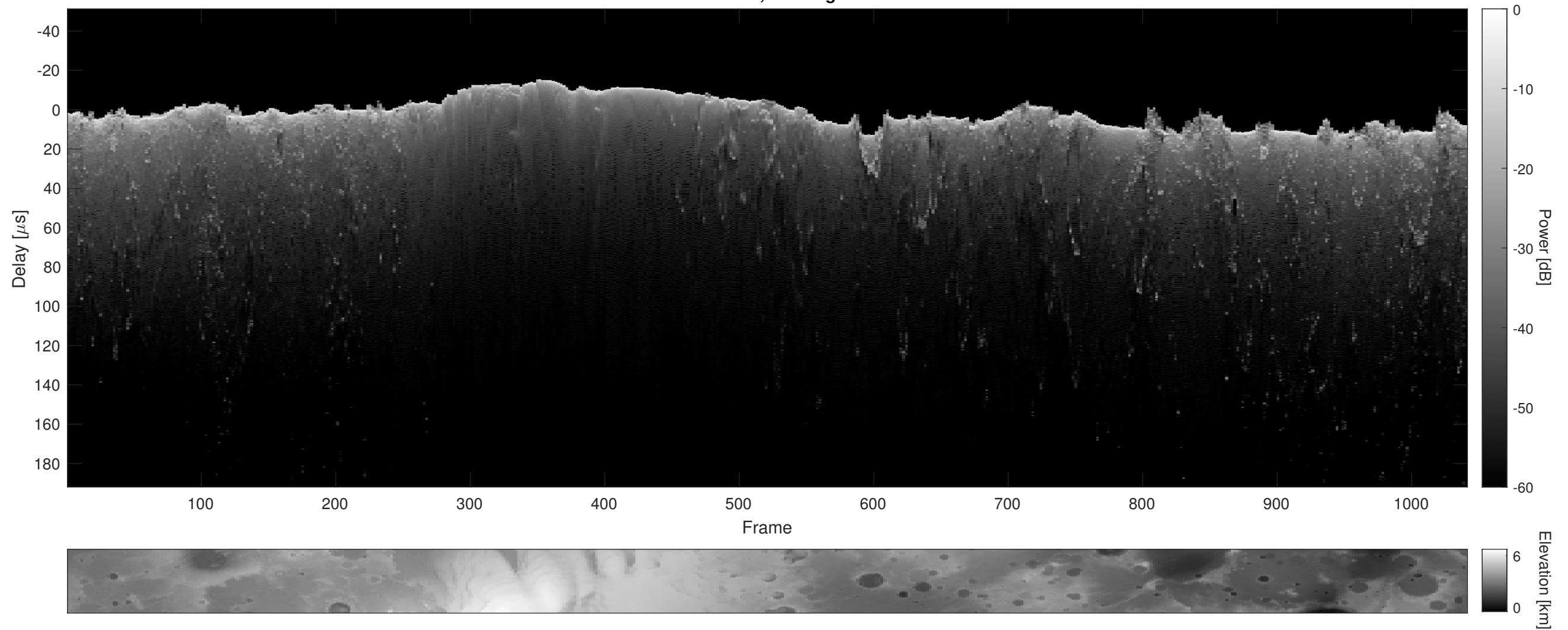
Orbit 10716, Cluttergram
