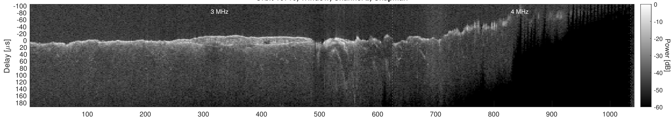
Orbit 10716, Window, Channel 2, Optimized
