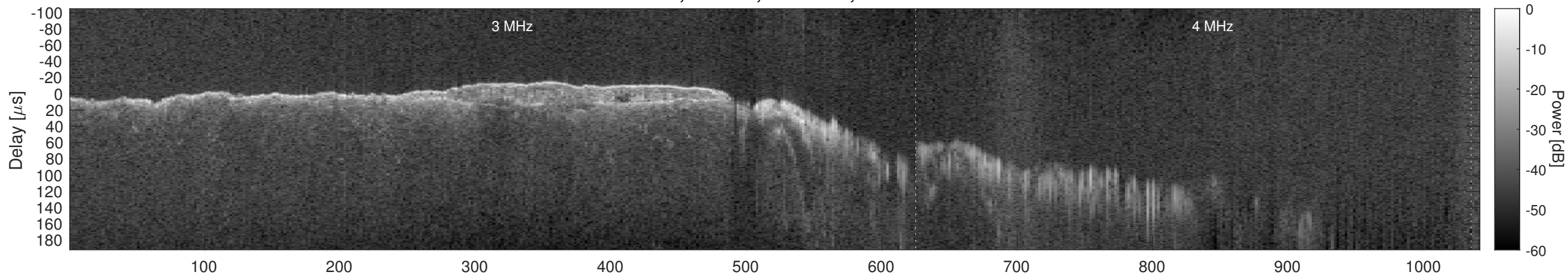
Orbit 10716, Window, Channel 2, Chapman
