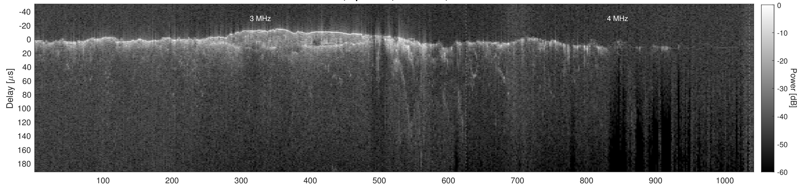
Orbit 10716, Cluttergram
