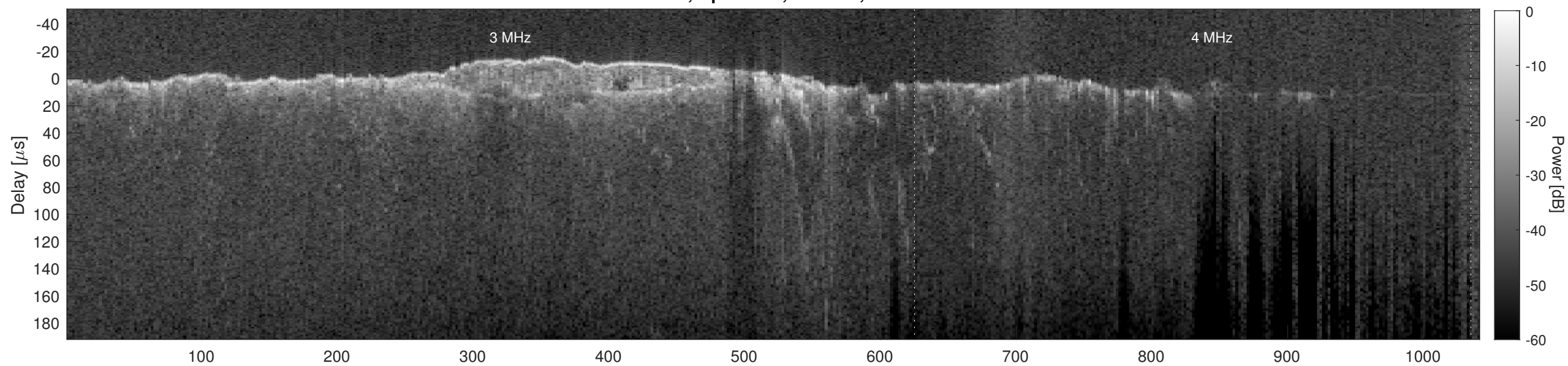
Orbit 10716, Cluttergram
