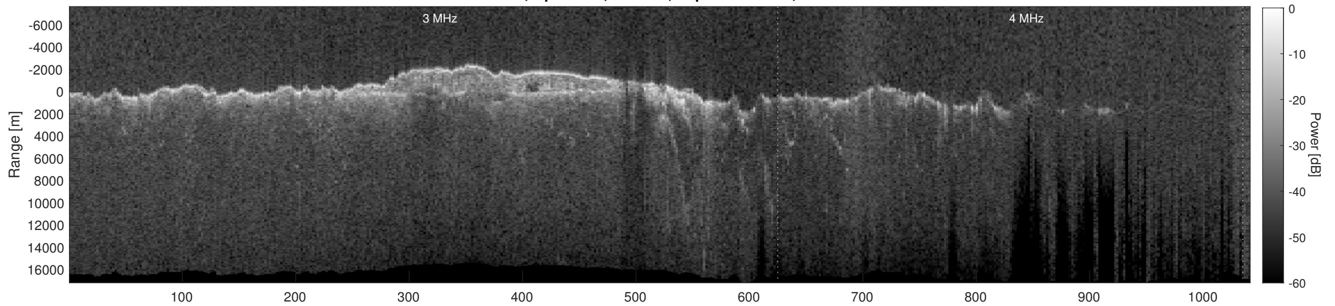
Orbit 10716, Depth-Corrected Cluttergram
