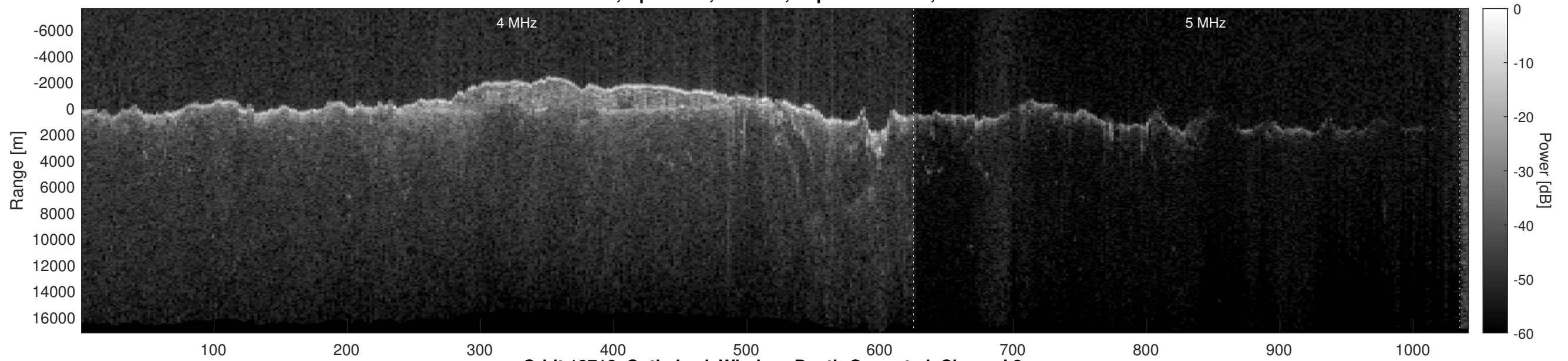
Orbit 10716, Optimized, Window, Depth-Corrected, Channel 2
