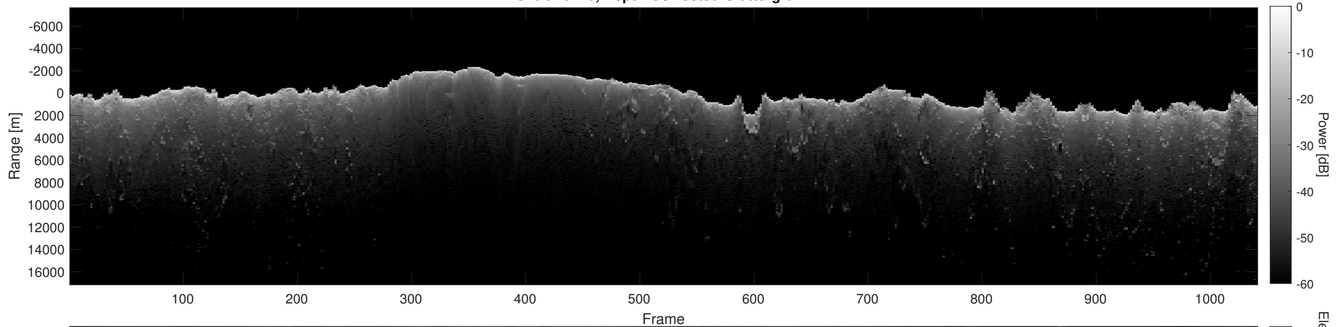
Orbit 10716, Depth-Corrected Cluttergram
