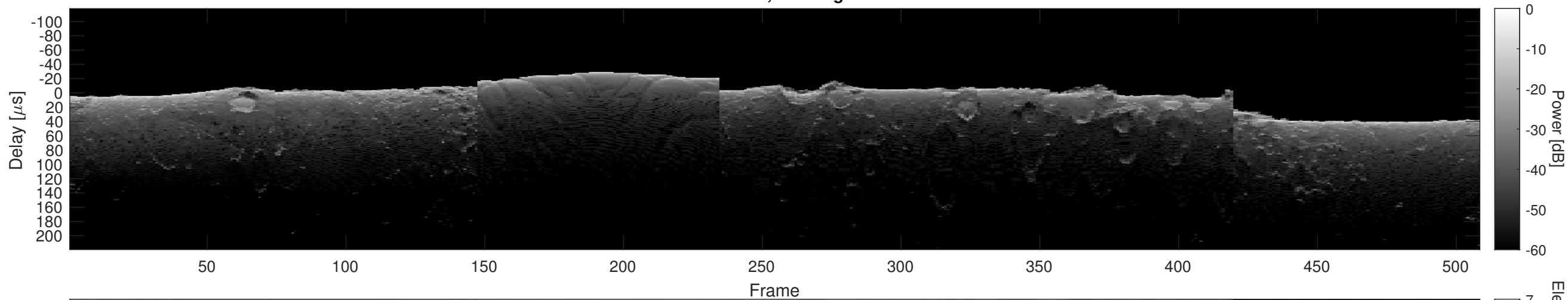
Orbit 10717, Cluttergram
