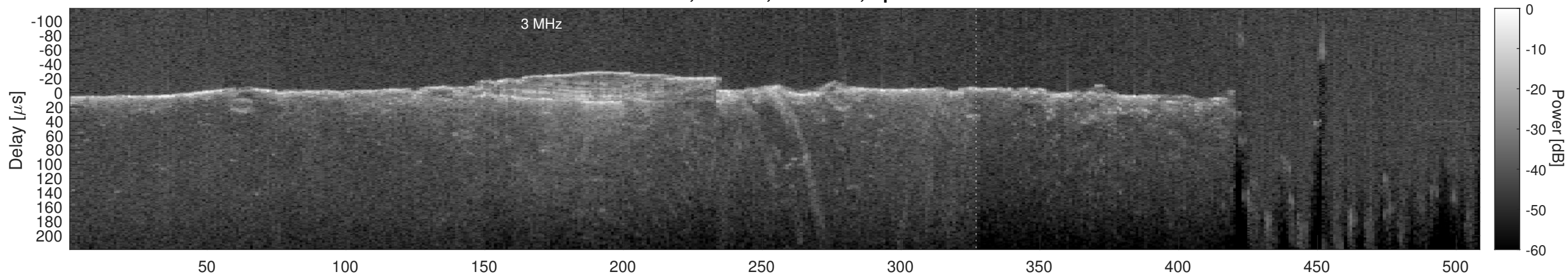
Orbit 10717, Cluttergram
