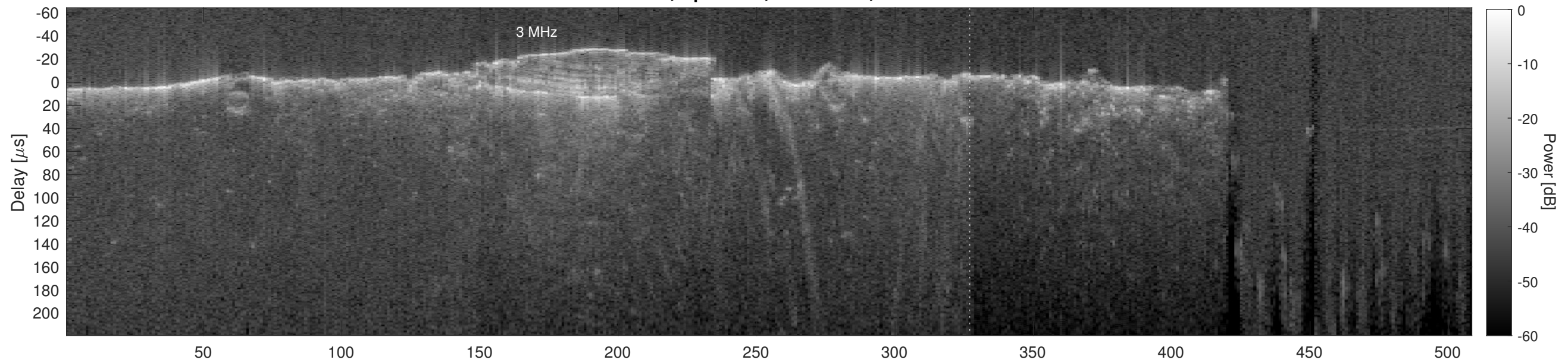
Orbit 10717, Cluttergram
