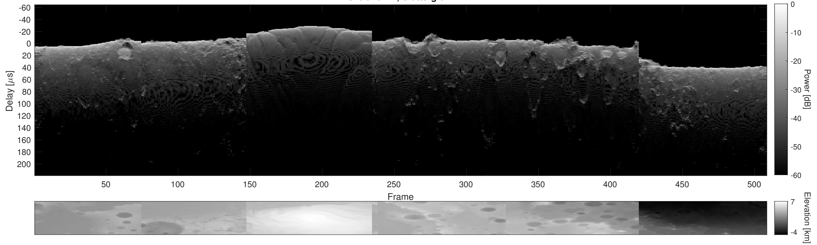
Orbit 10717, Cluttergram
