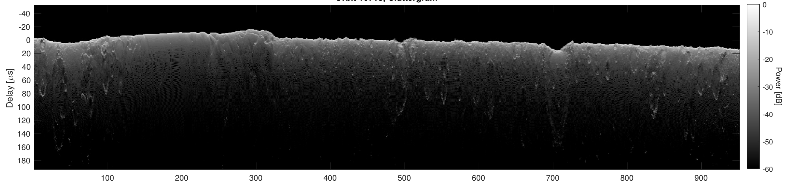
Orbit 10718, Cluttergram
