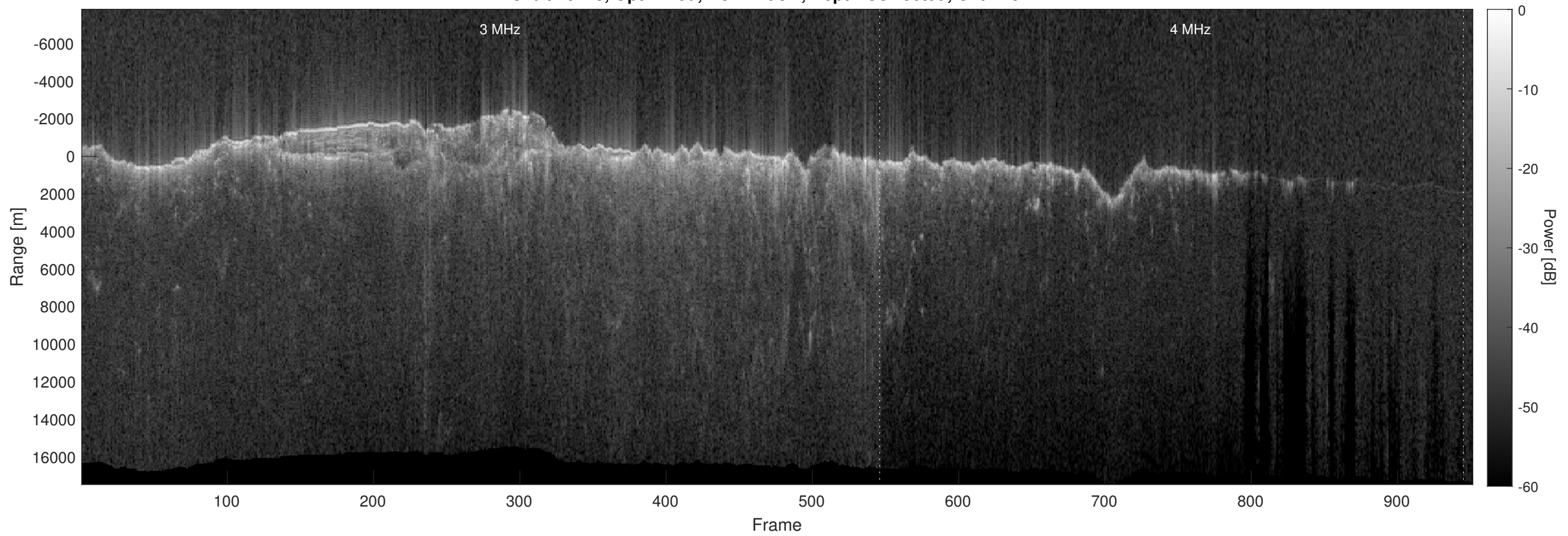
Orbit 10718, Optimized, No Window, Depth-Corrected, Channel 2
