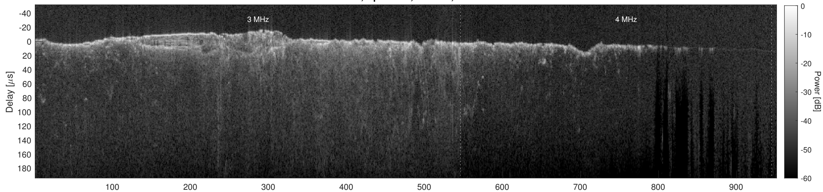
Orbit 10718, Cluttergram
