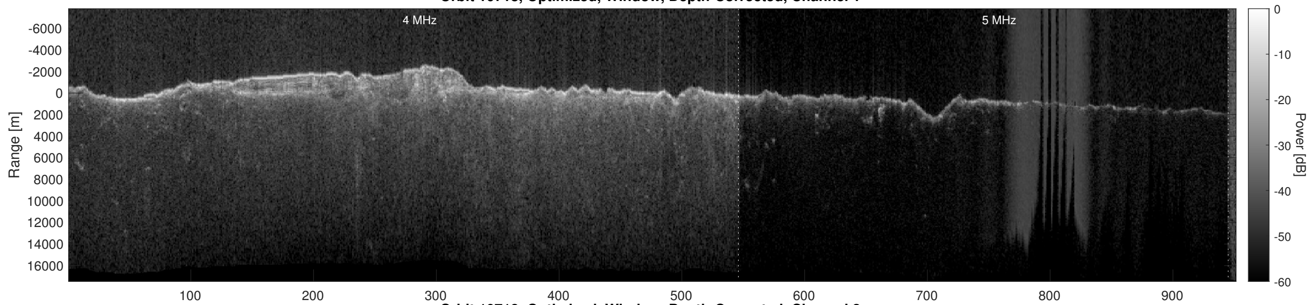
Orbit 10718, Optimized, Window, Depth-Corrected, Channel 2
