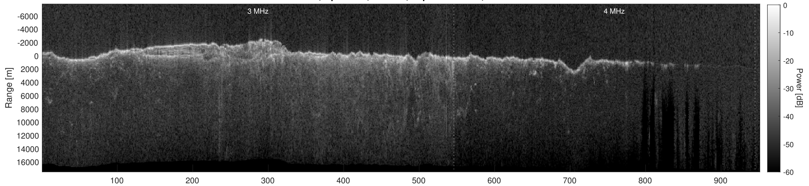
Orbit 10718, Depth-Corrected Cluttergram
