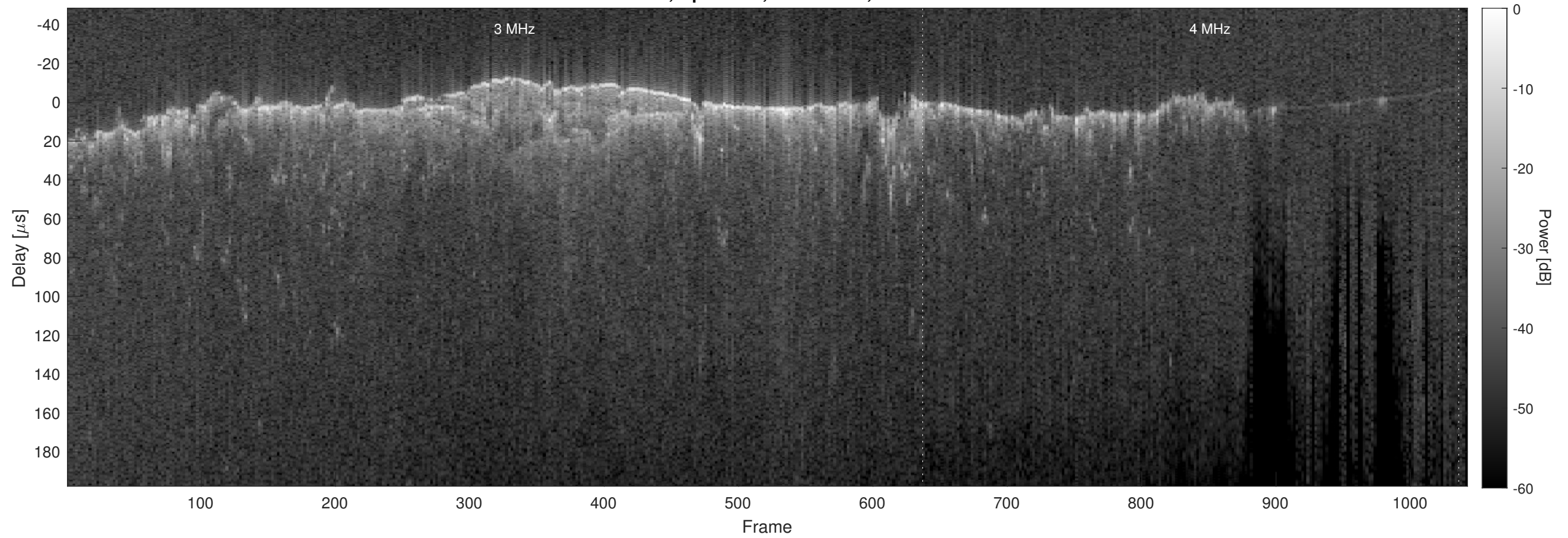
Orbit 10719, Optimized, No Window, Channel 2
