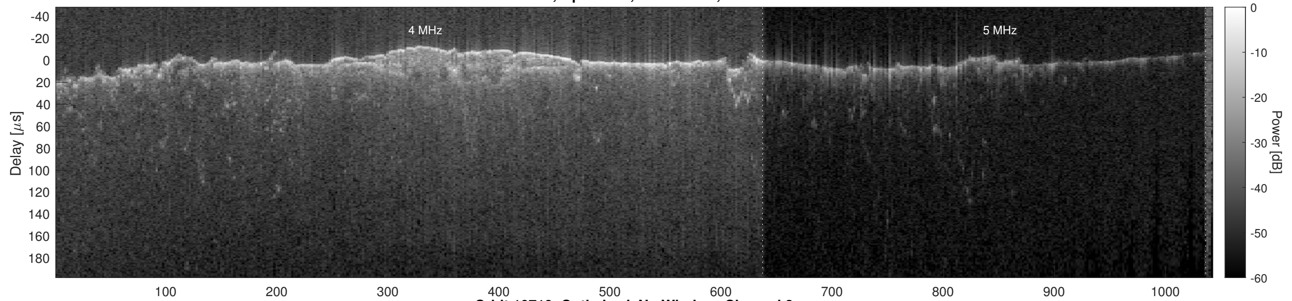
Orbit 10719, Optimized, No Window, Channel 2
