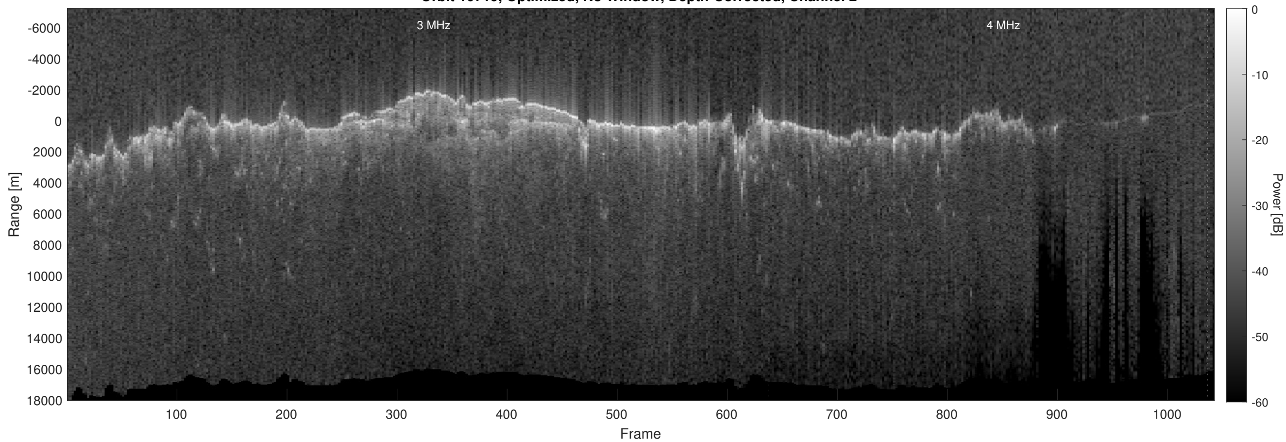
Orbit 10719, Optimized, No Window, Depth-Corrected, Channel 2
