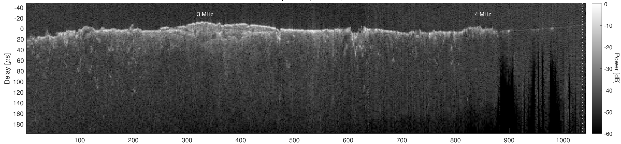
Orbit 10719, Cluttergram
