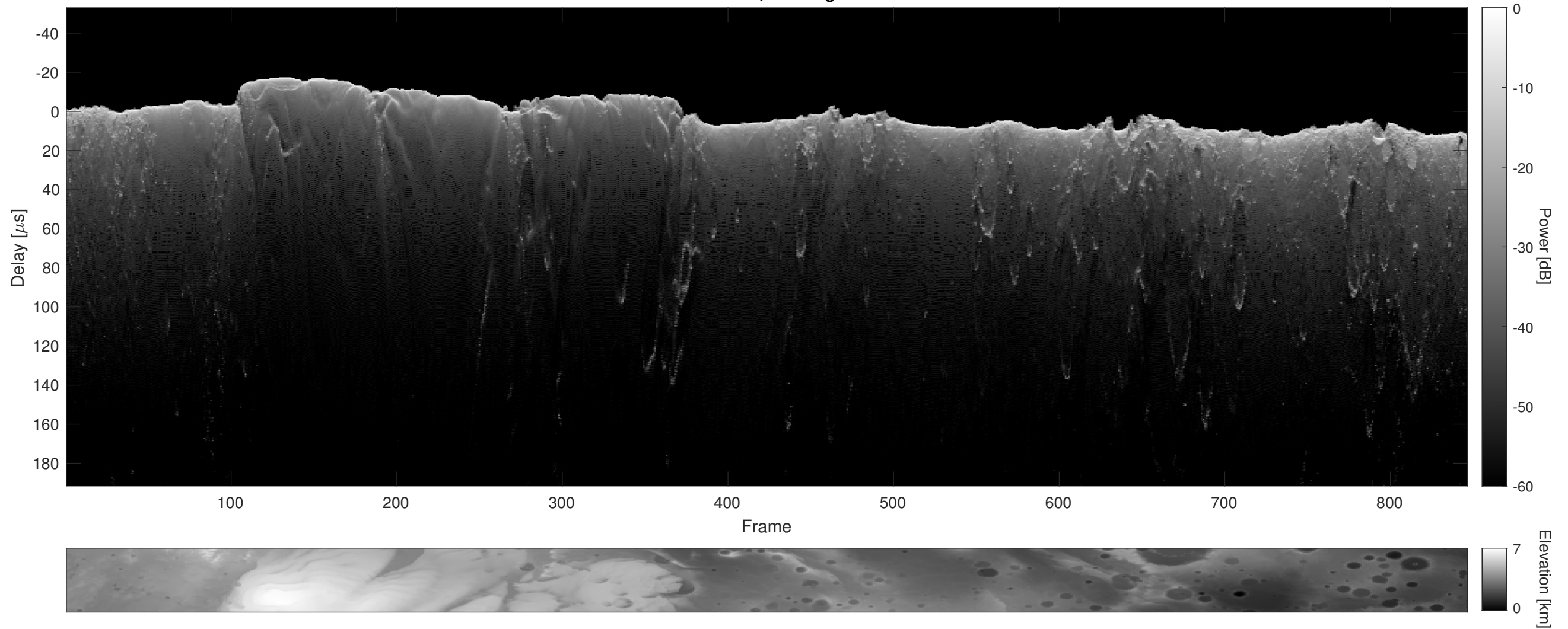
Orbit 10720, Cluttergram
