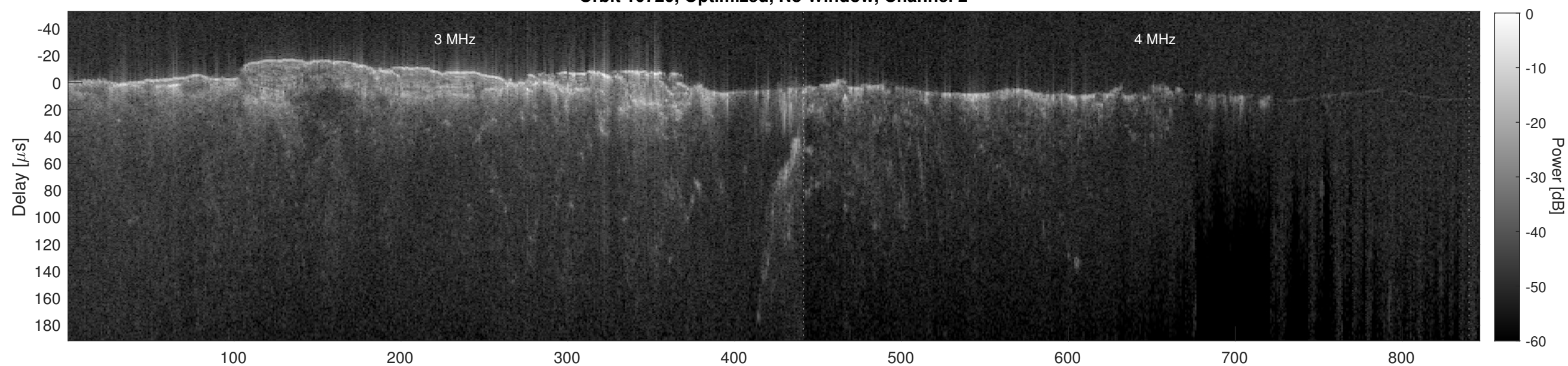
Orbit 10720, Cluttergram
