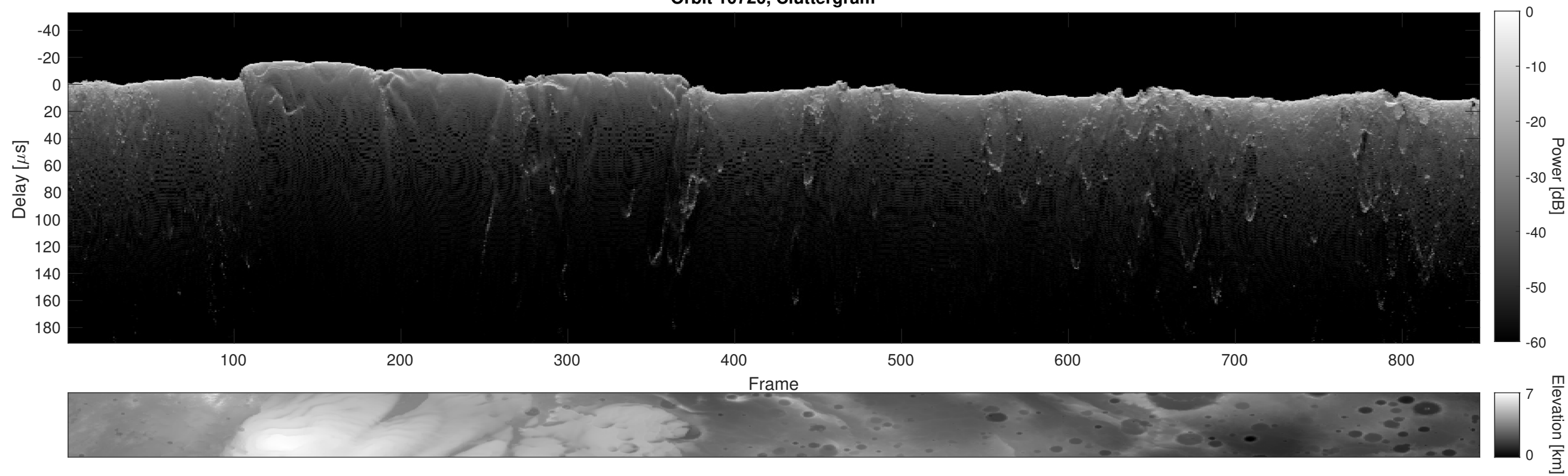
Orbit 10720, Cluttergram
