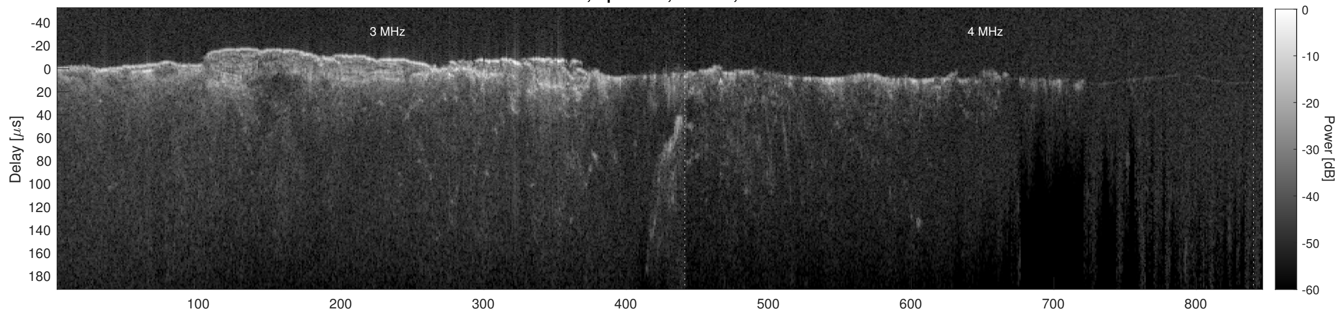
Orbit 10720, Cluttergram
