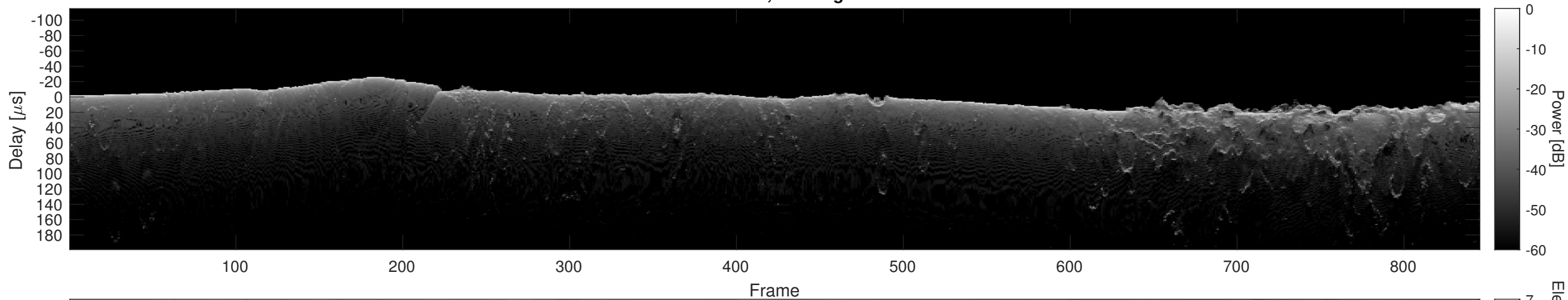
Orbit 10721, Cluttergram
