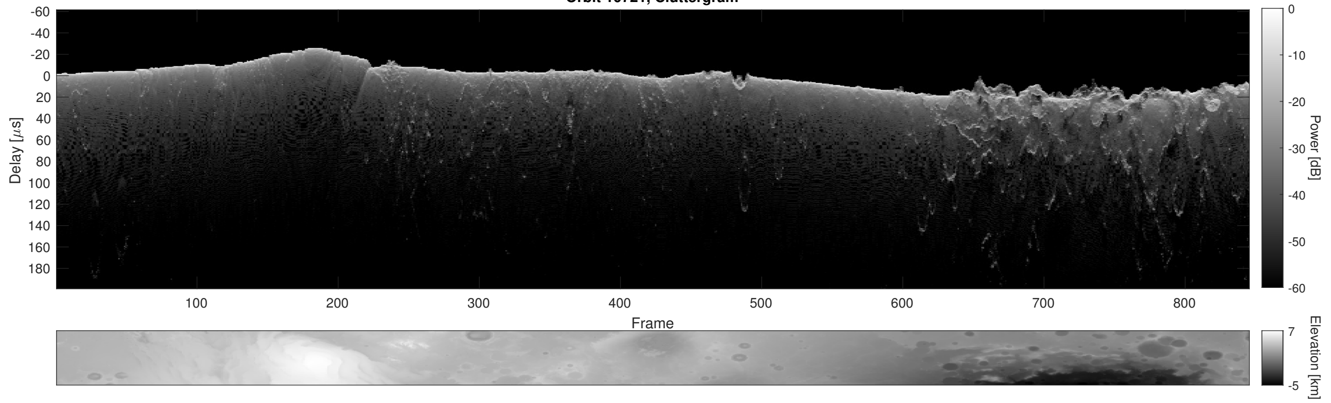
Orbit 10721, Cluttergram
