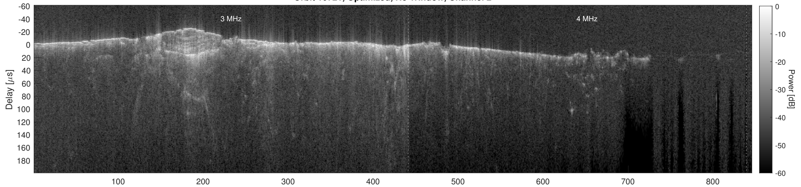
Orbit 10721, Cluttergram
