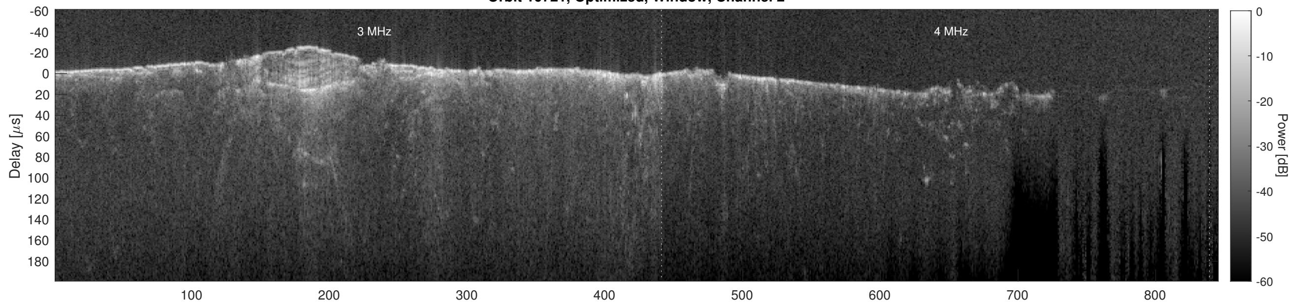
Orbit 10721, Cluttergram
