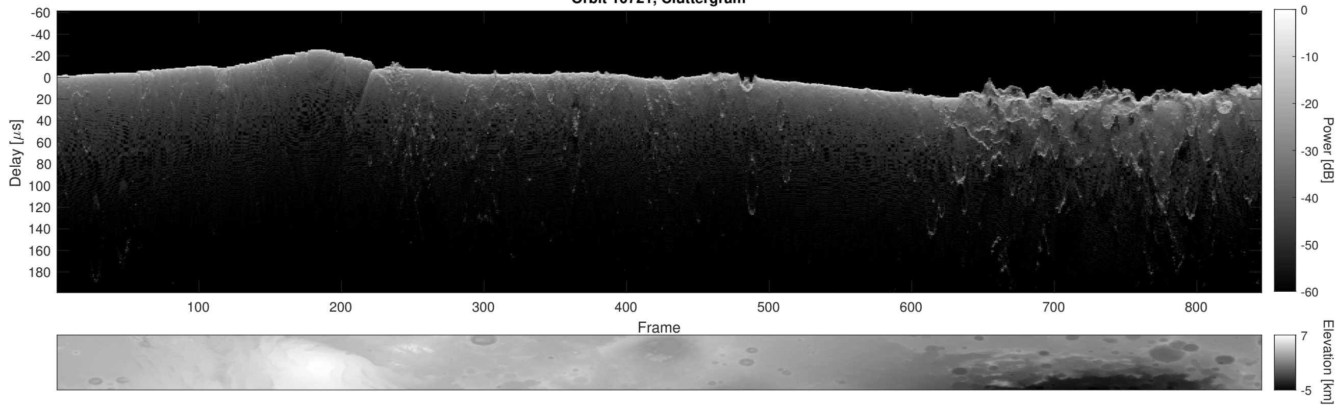
Orbit 10721, Cluttergram
