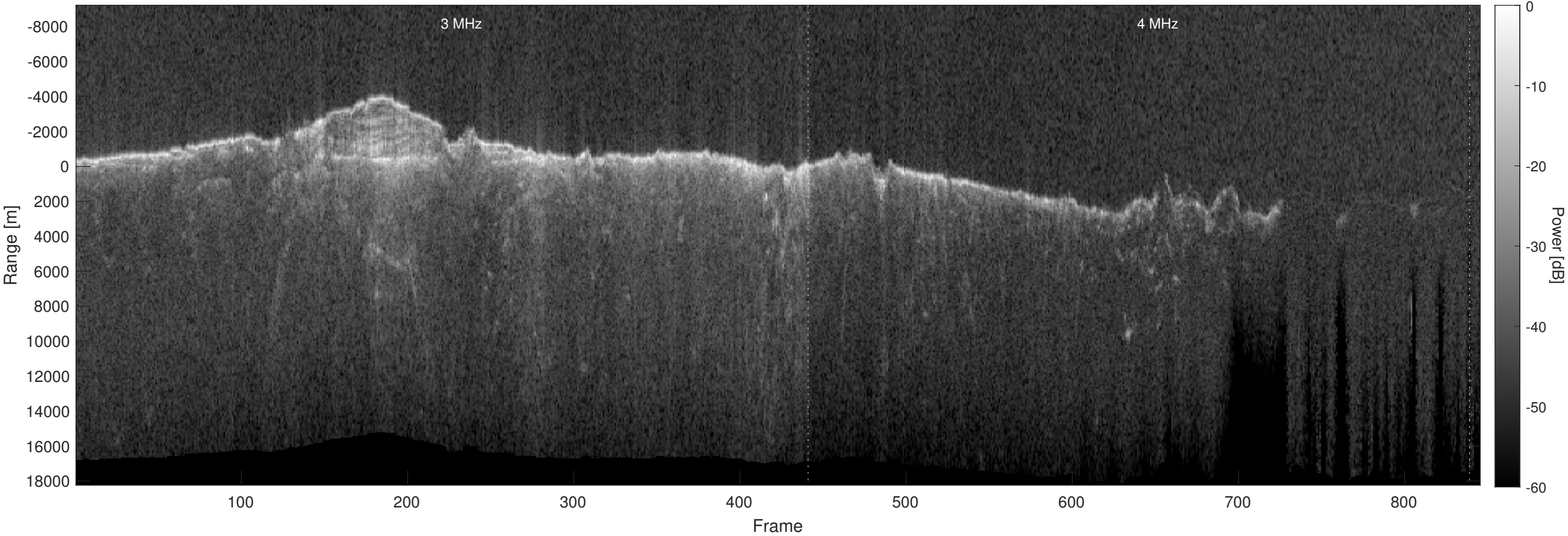
Orbit 10721, Optimized, Window, Depth-Corrected, Channel 2
