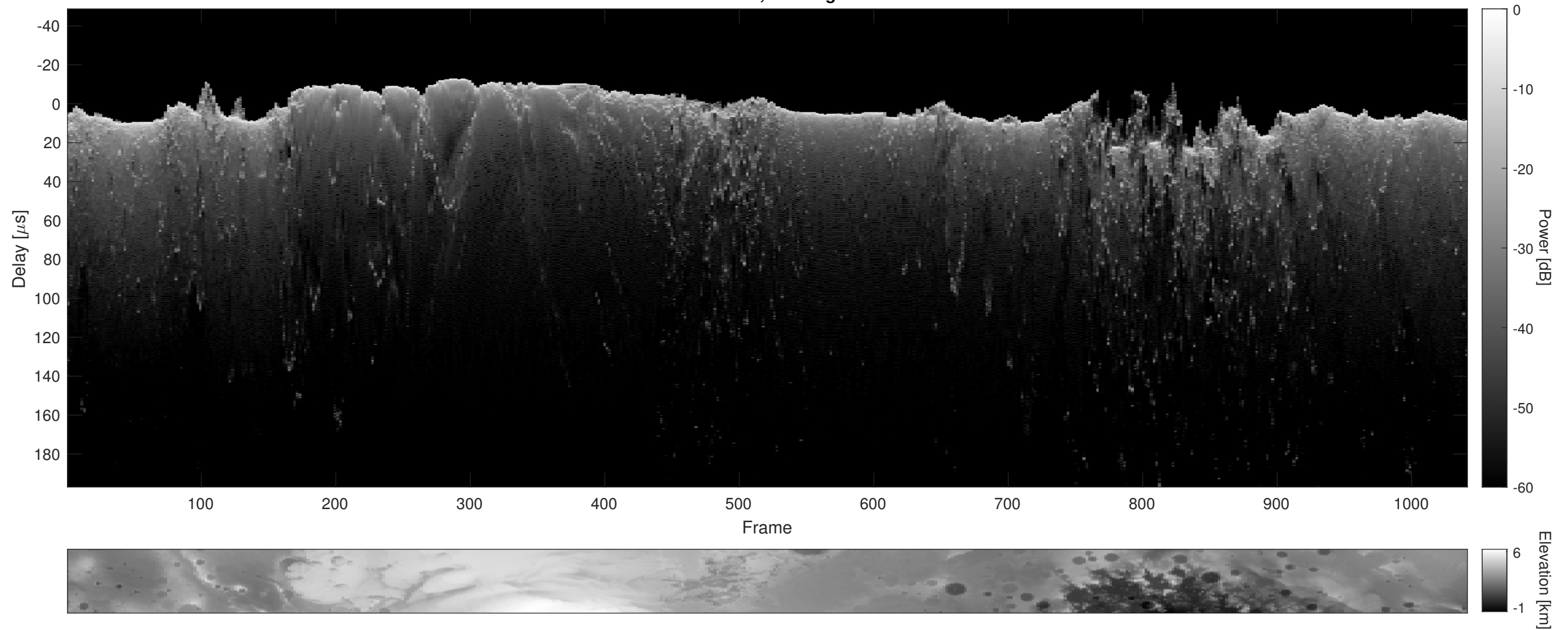
Orbit 10722, Cluttergram
