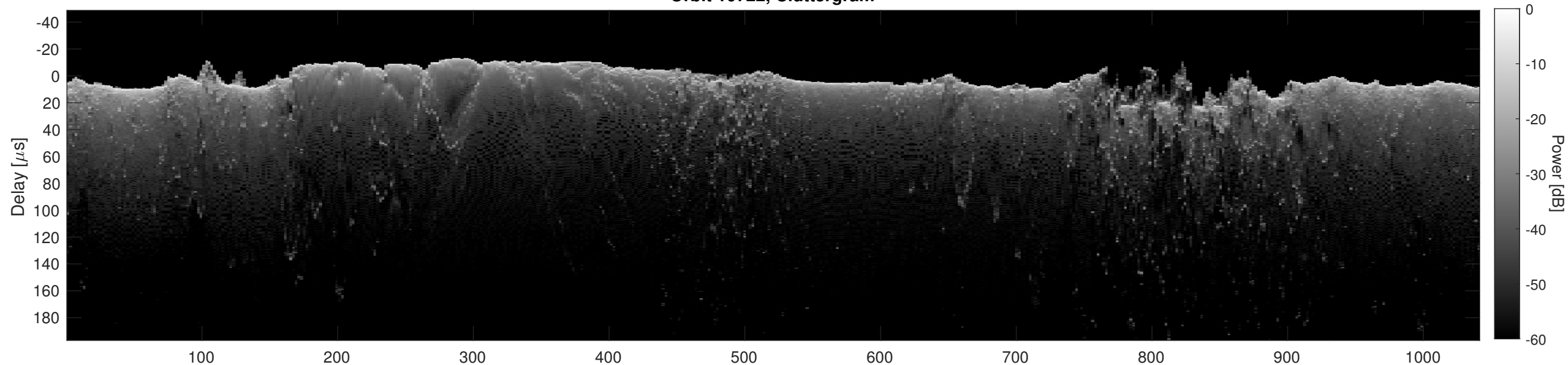
Orbit 10722, Cluttergram
