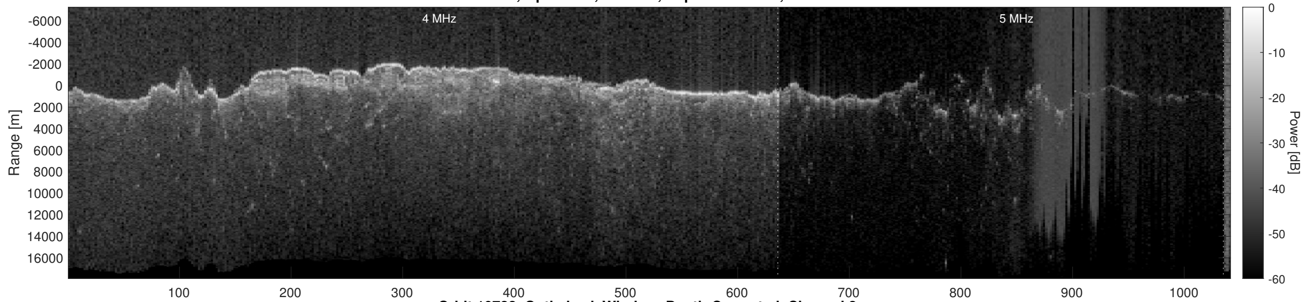
Orbit 10722, Optimized, Window, Depth-Corrected, Channel 2
