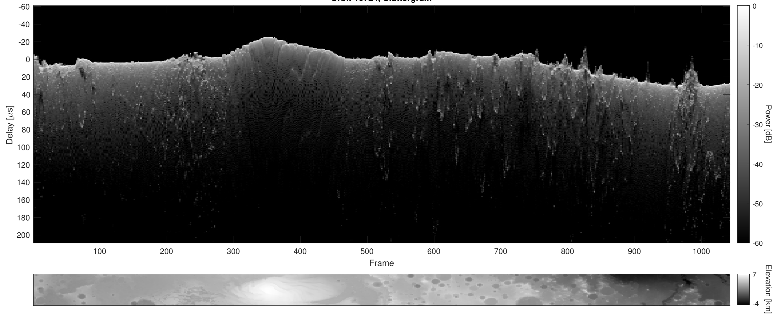
Orbit 10724, Cluttergram
