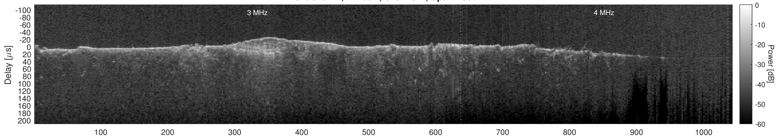
Orbit 10724, Cluttergram
