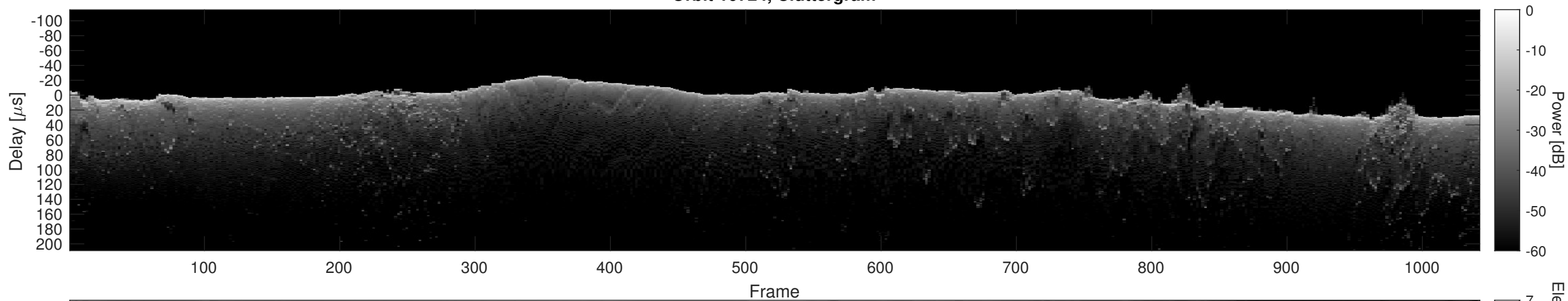
Orbit 10724, Cluttergram
