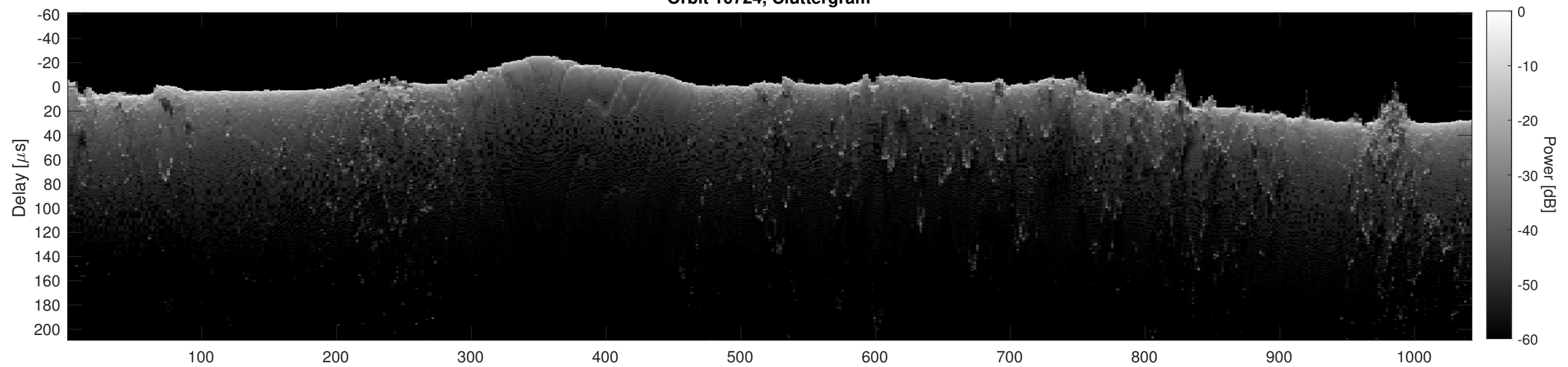
Orbit 10724, Cluttergram
