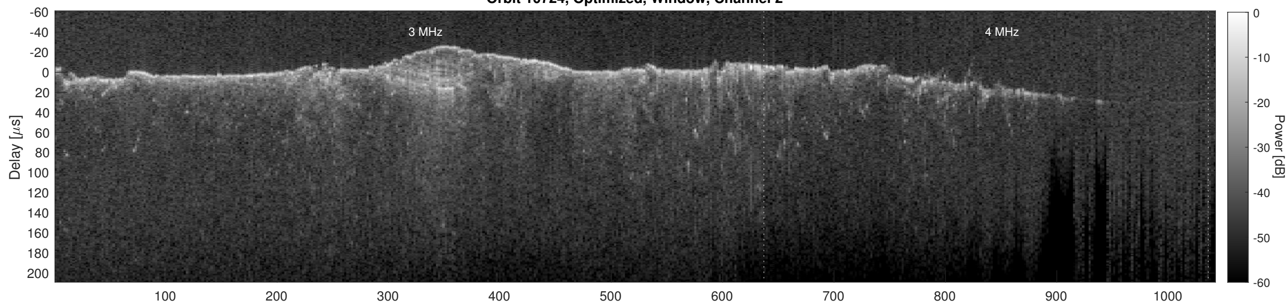
Orbit 10724, Cluttergram
