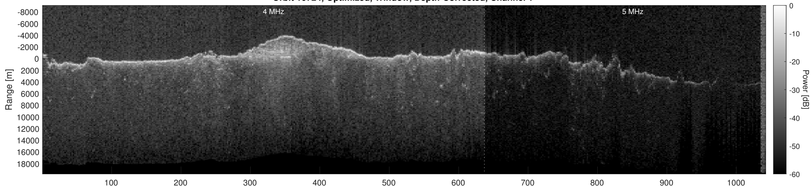
Orbit 10724, Optimized, Window, Depth-Corrected, Channel 2
