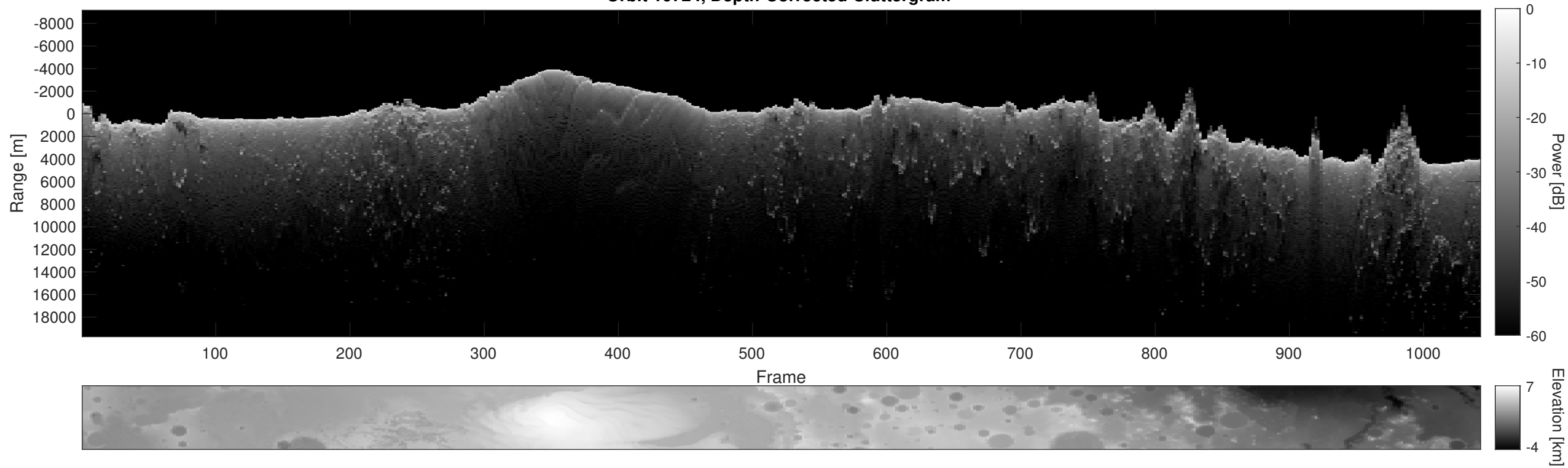
Orbit 10724, Depth-Corrected Cluttergram
