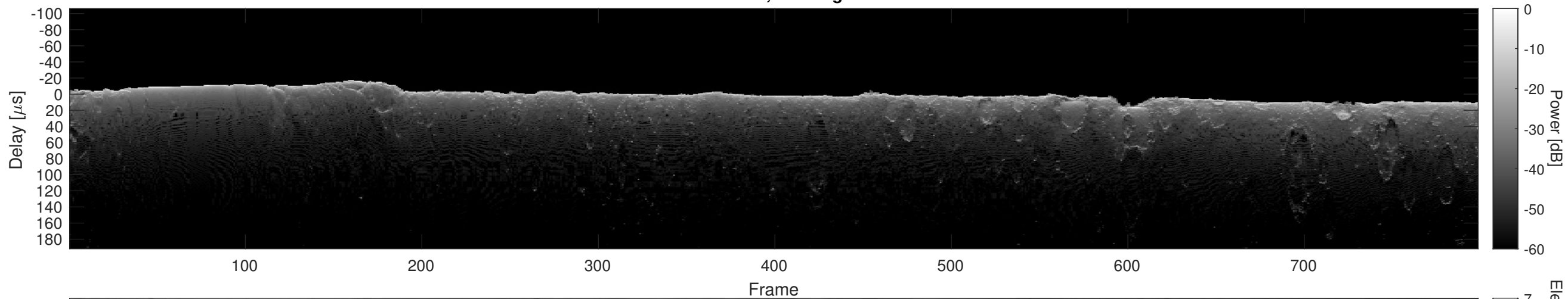
Orbit 10725, Cluttergram
