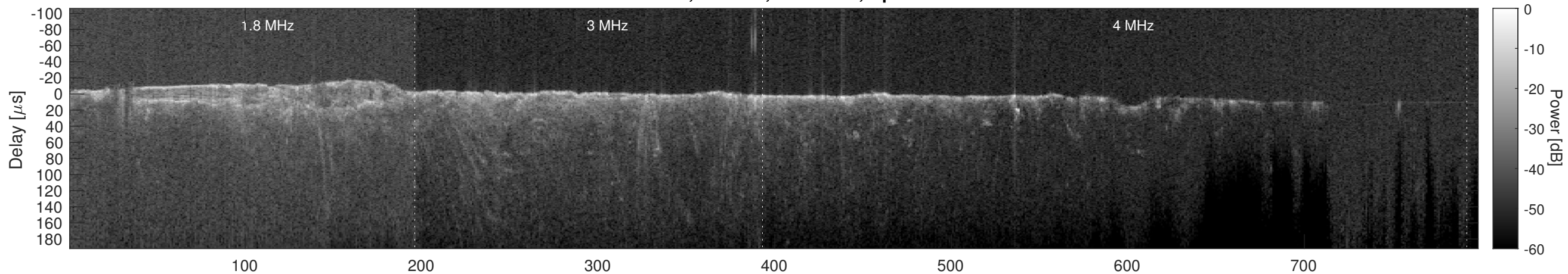
Orbit 10725, Cluttergram
