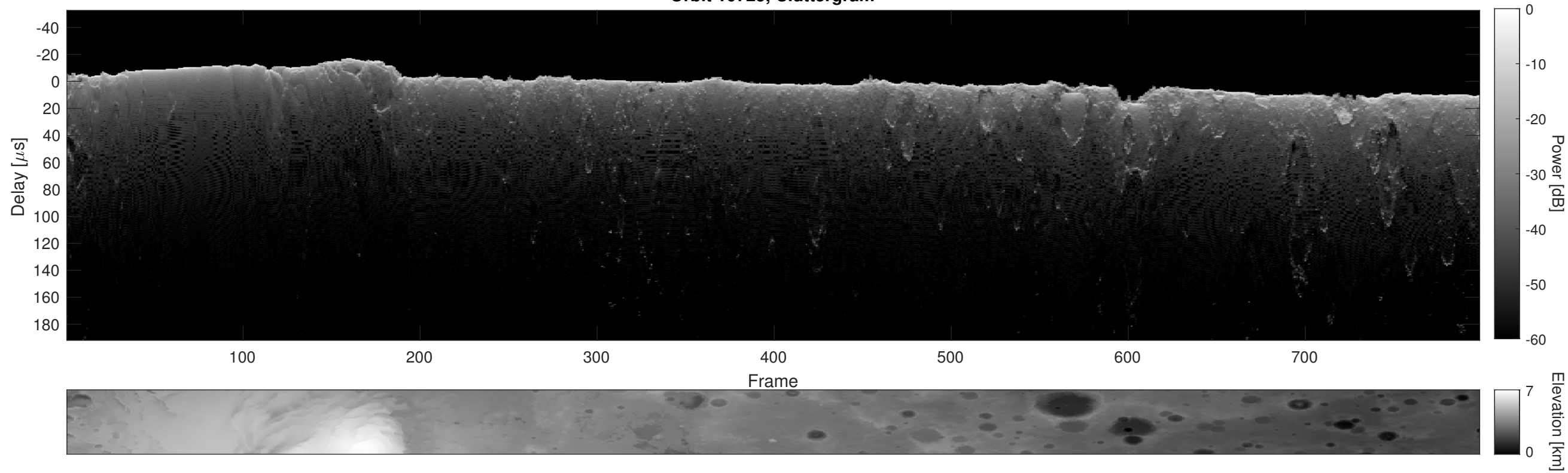
Orbit 10725, Cluttergram
