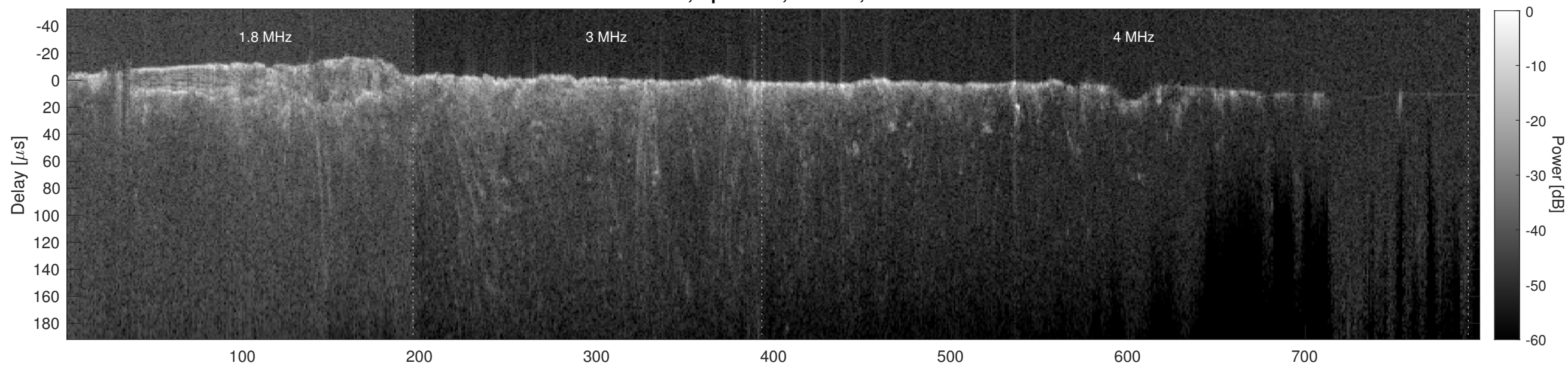
Orbit 10725, Cluttergram
