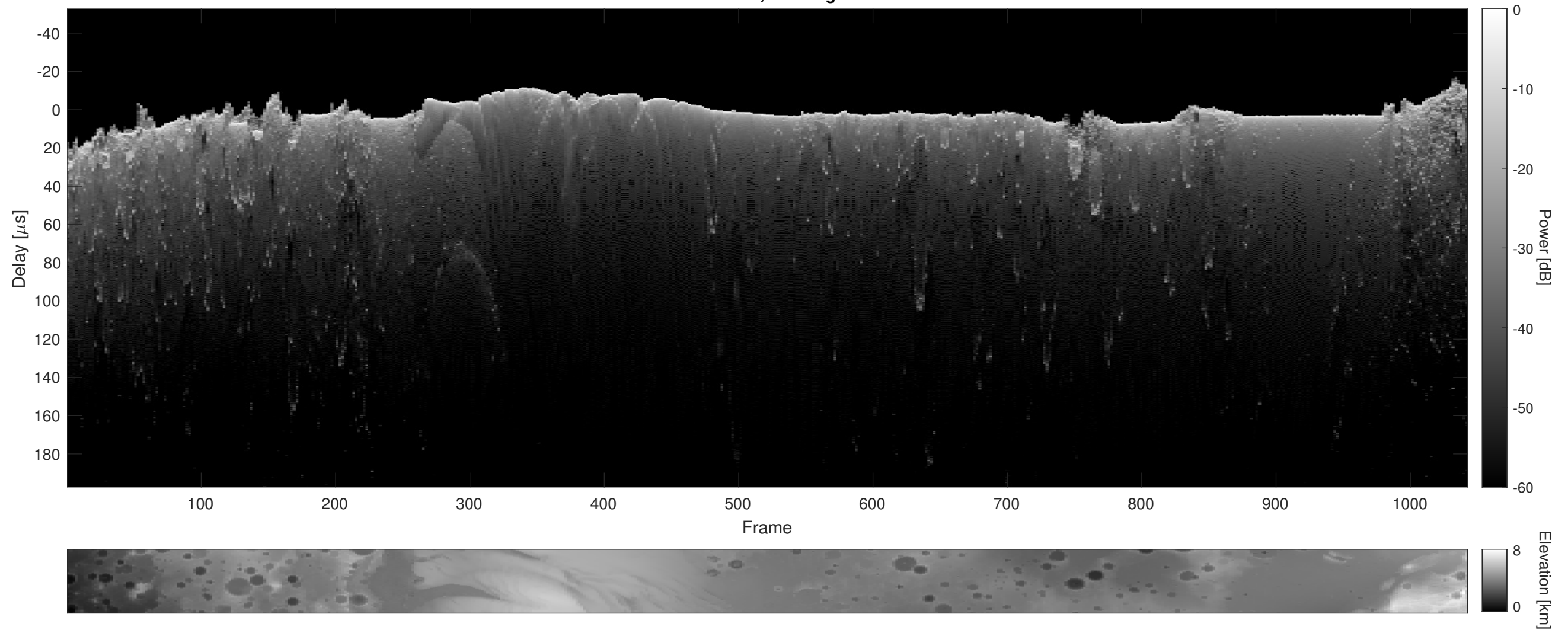
Orbit 10726, Cluttergram
