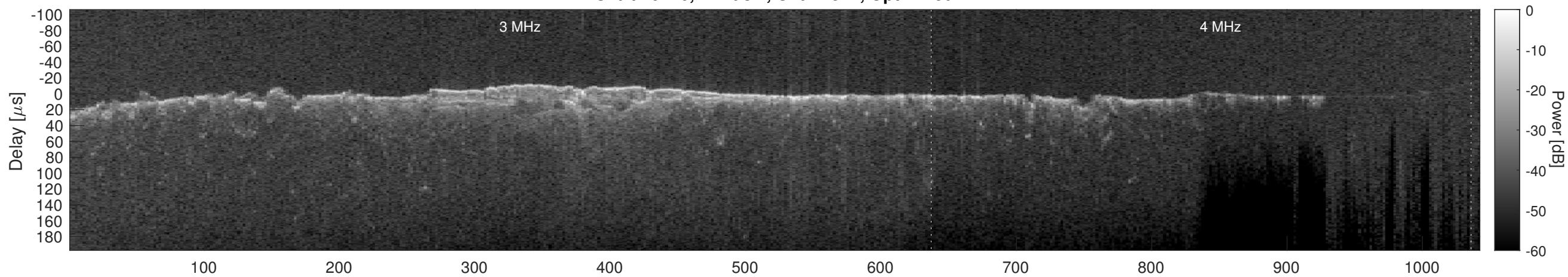
Orbit 10726, Cluttergram
