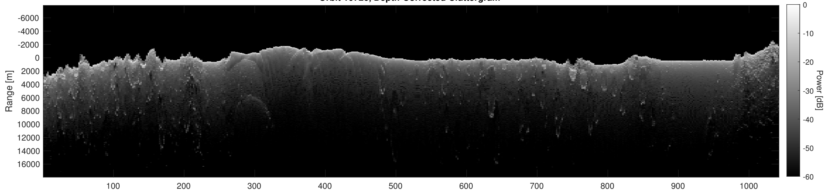
Orbit 10726, Depth-Corrected Cluttergram
