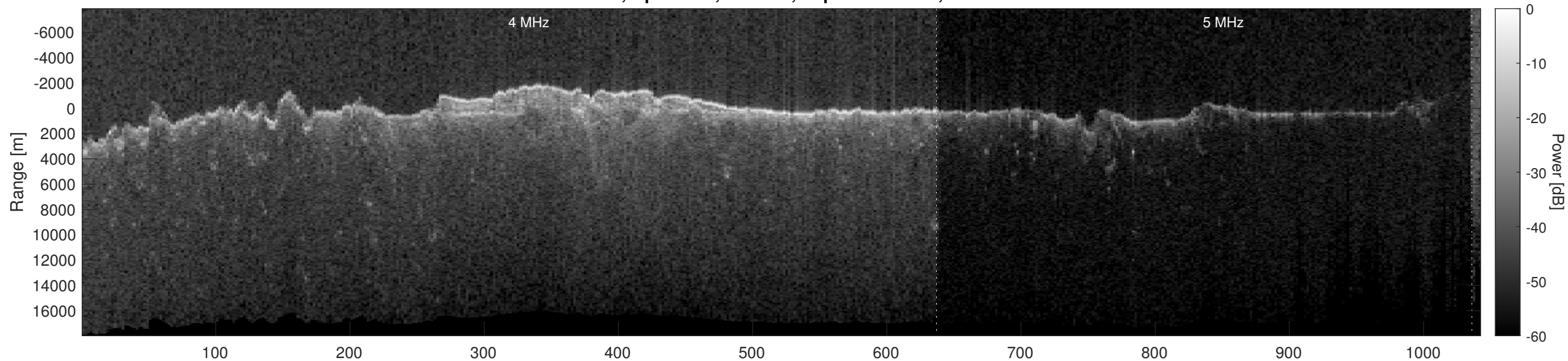
Orbit 10726, Optimized, Window, Depth-Corrected, Channel 2
