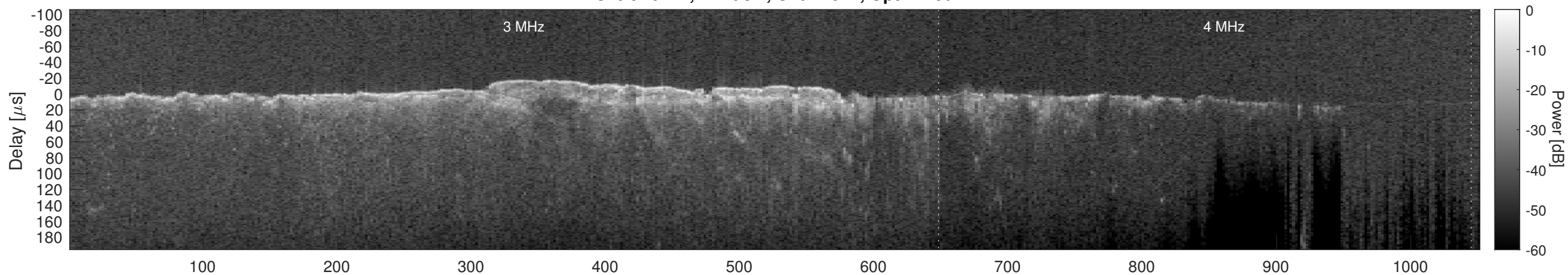
Orbit 10727, Cluttergram
