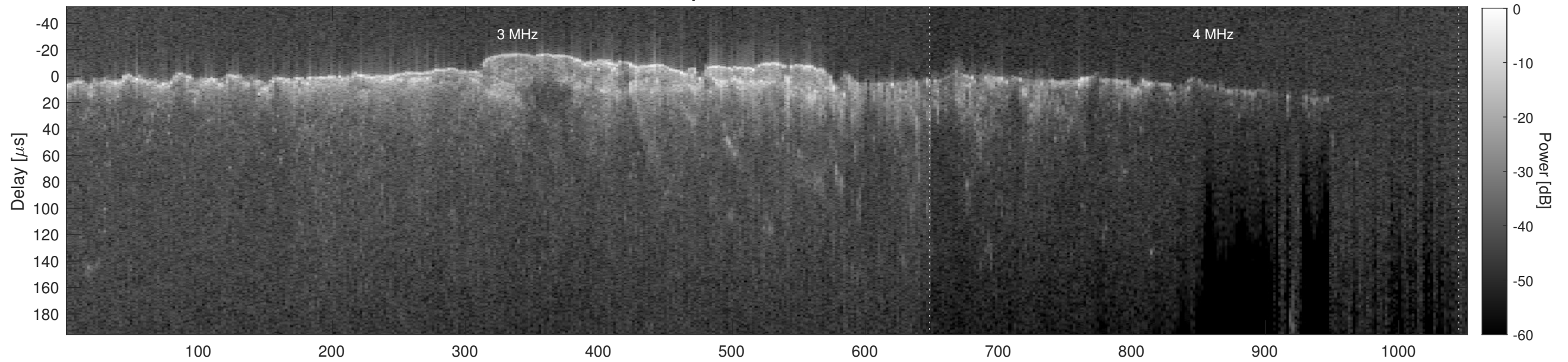
Orbit 10727, Cluttergram
