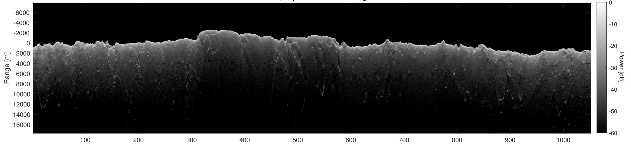
Orbit 10727, Depth-Corrected Cluttergram
