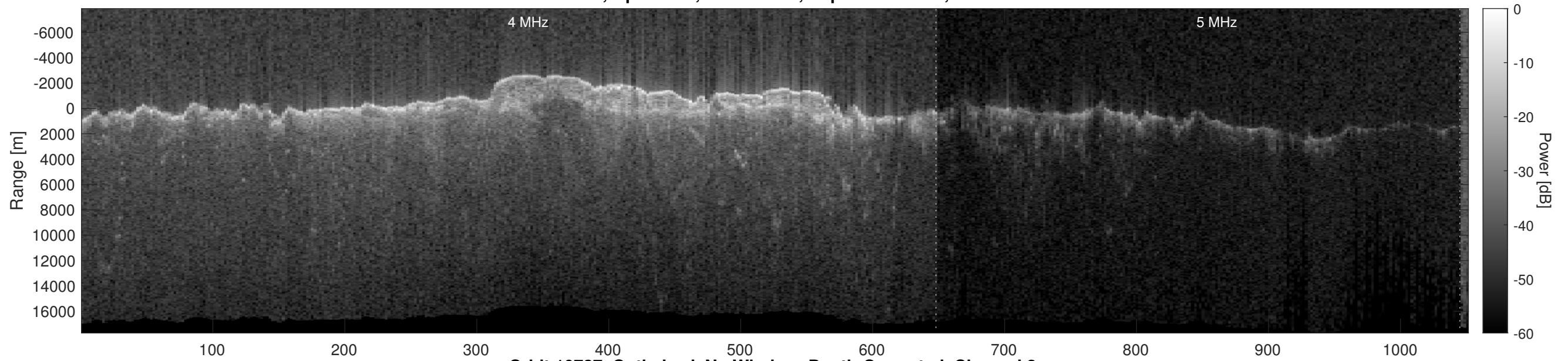
Orbit 10727, Optimized, No Window, Depth-Corrected, Channel 2
