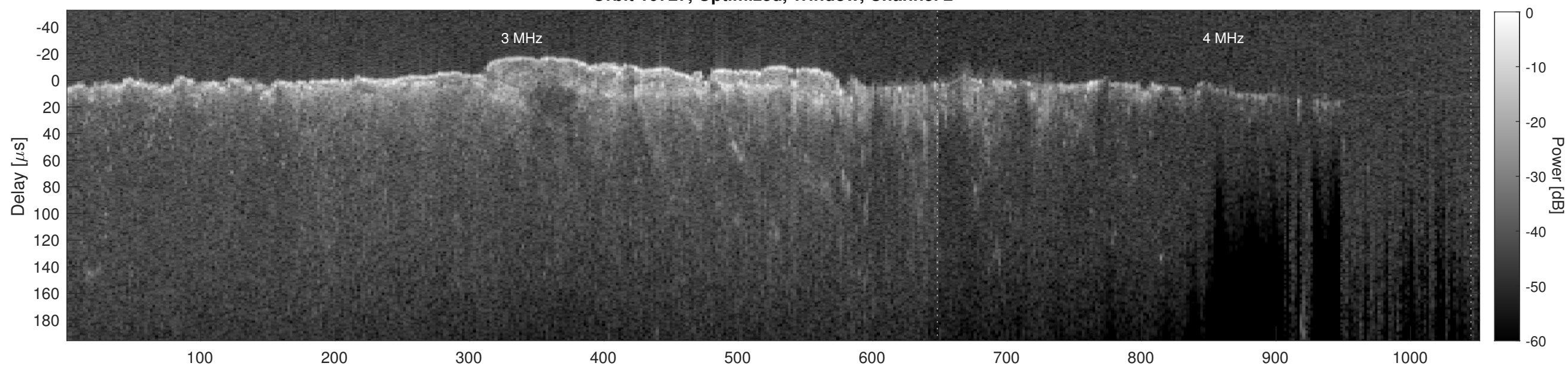
Orbit 10727, Cluttergram
