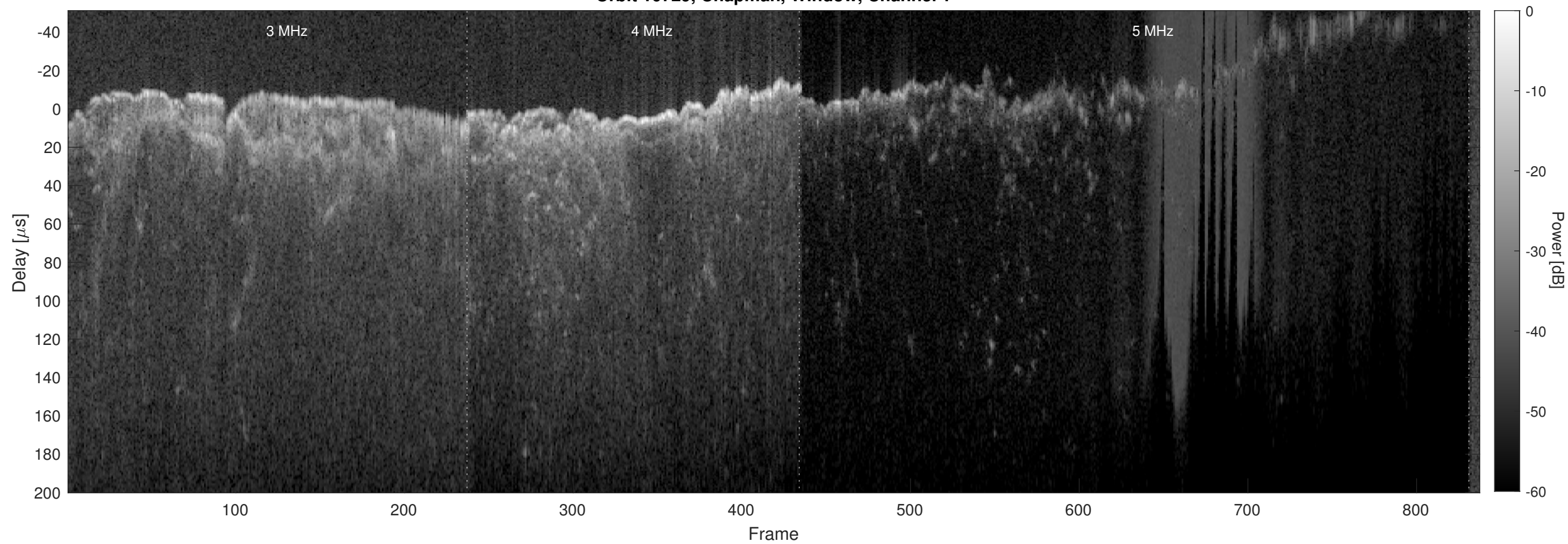
Orbit 10729, Chapman, Window, Channel 2
