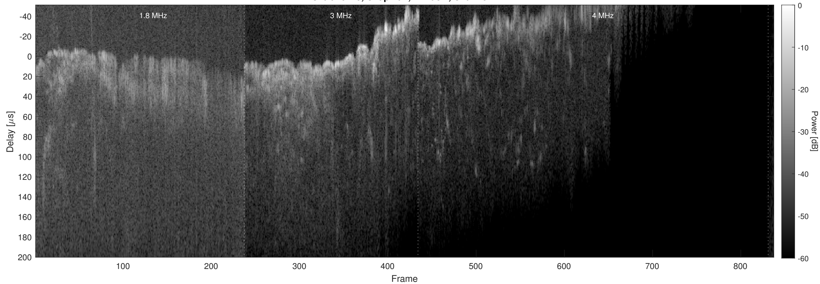
Orbit 10729, Chapman, Window, Channel 2
