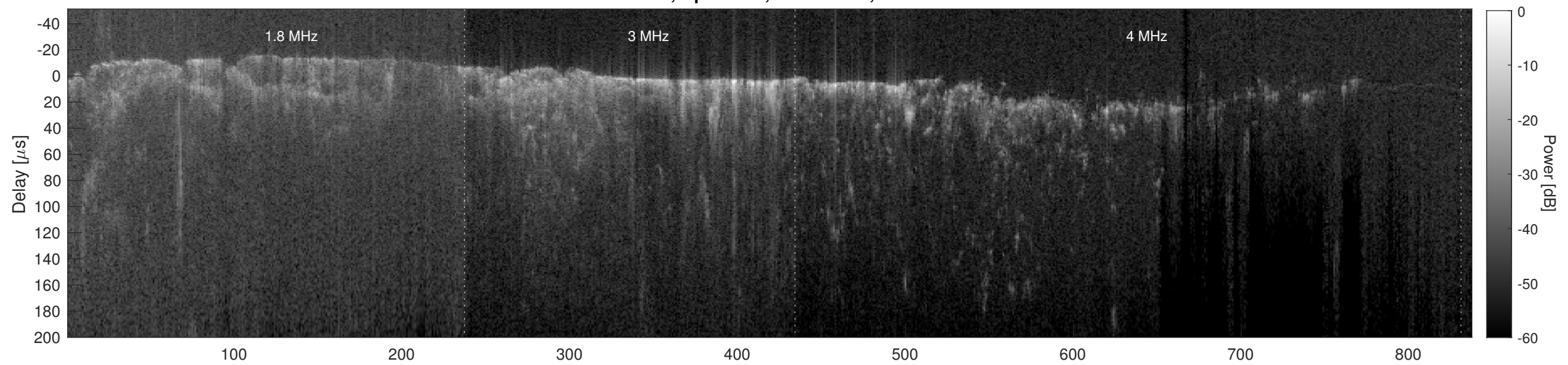
Orbit 10729, Cluttergram
