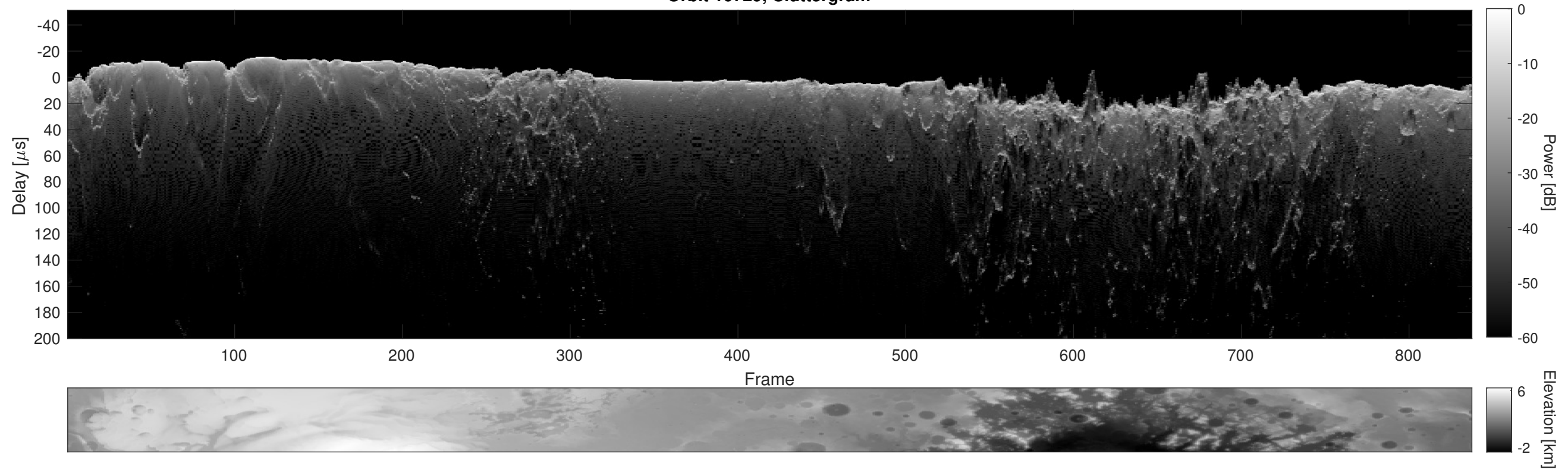
Orbit 10729, Cluttergram
