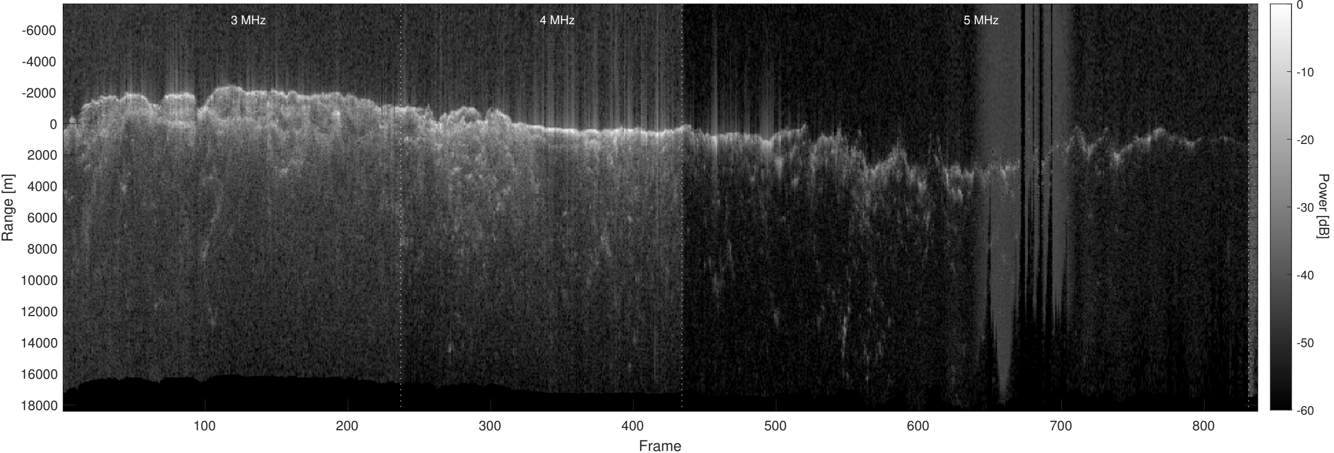
Orbit 10729, Optimized, No Window, Depth-Corrected, Channel 2
