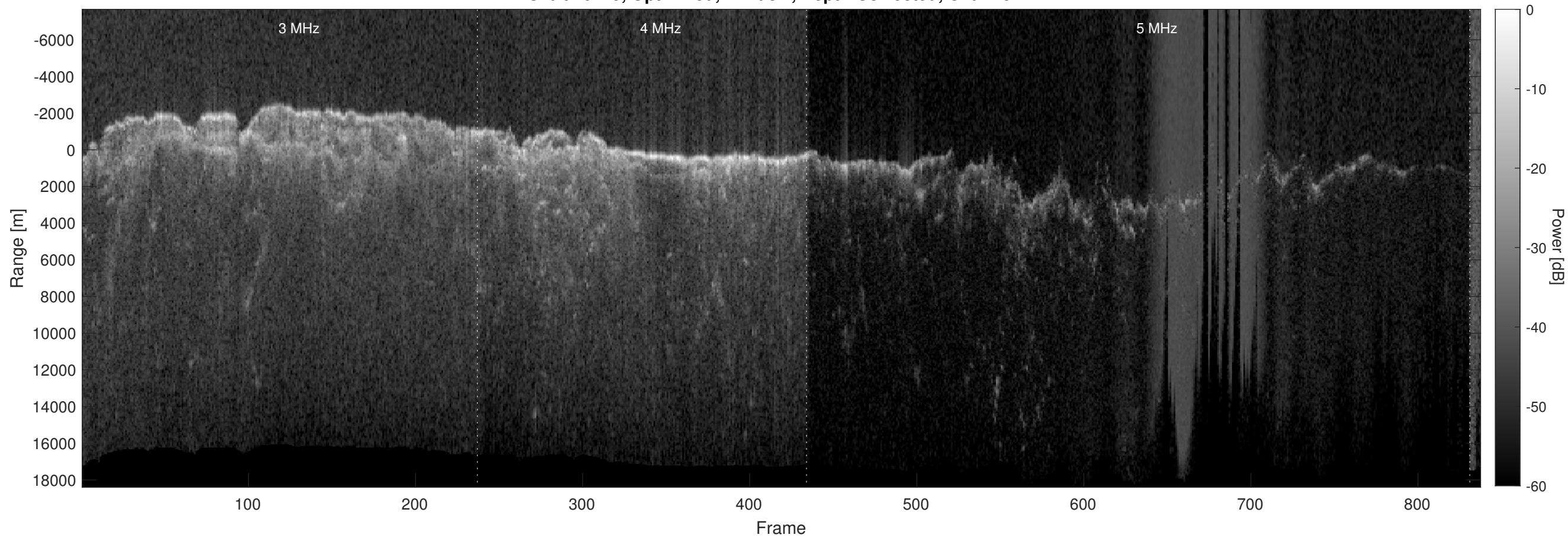
Orbit 10729, Optimized, Window, Depth-Corrected, Channel 2
