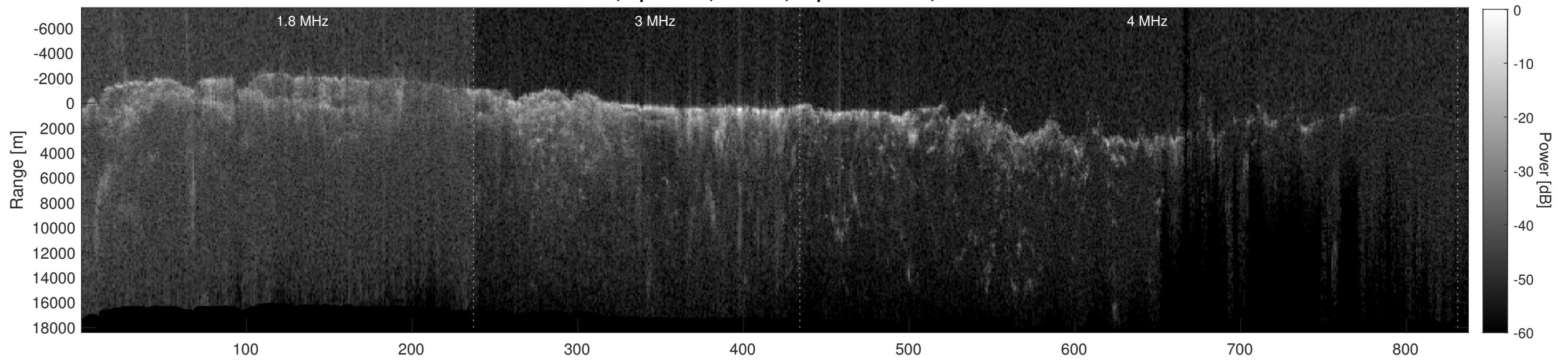
Orbit 10729, Depth-Corrected Cluttergram
