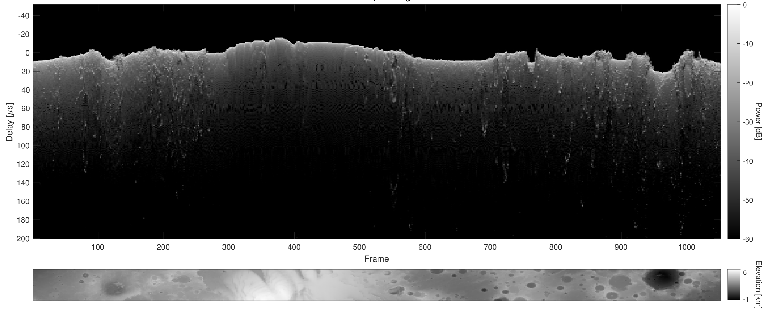
Orbit 10730, Cluttergram
