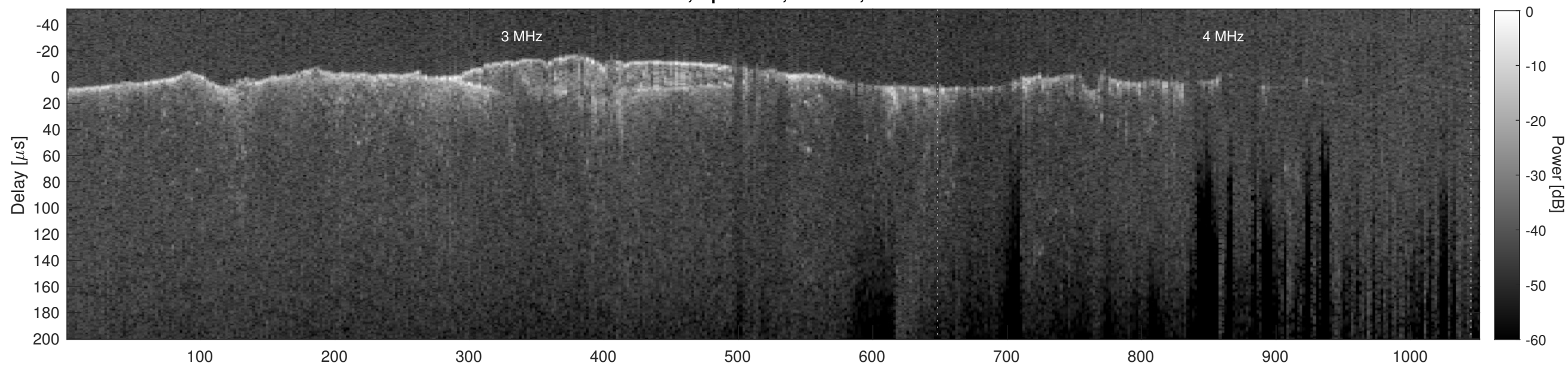
Orbit 10730, Cluttergram
